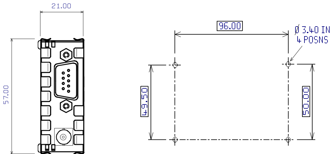
FIXING CENTRES FOR ENCLOSURE PLAN VIEW
